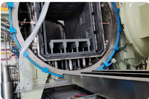
Reaction Sintering Furnace for Silicon Carbide image 2
