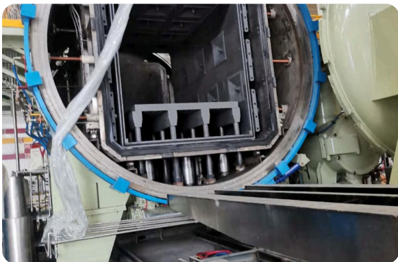
Recrystallization Sintering Furnace for Silicon Carbide image 2
