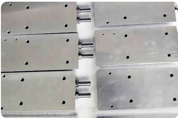
Water-Cooled Silicon Sleeve Heat Sink for Thyristors image 2
